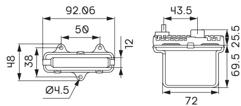
Control unit
