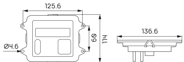
Control unit
